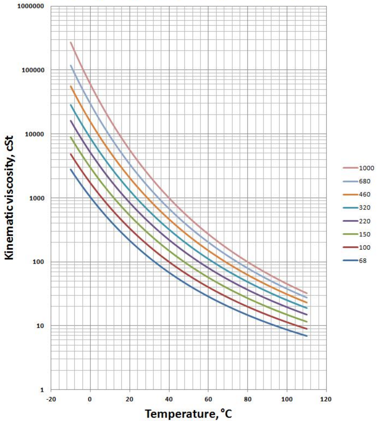
Viscosity - Temperature Diagram for Omala S2 G
